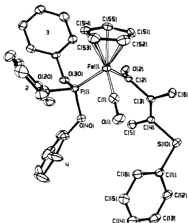
Figure 2. ORTEP diagram showing the crystal and molecular structure of CpFeCO[P(OPh) 3 ]( \eta^1 -( E )-C(O)C(Me)=C(Me)SPh) (1).
