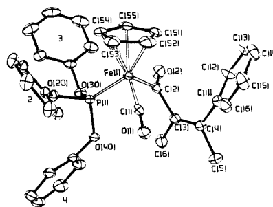
Figure 1. ORTEP diagram showing the crystal and molecular structure of CpFeCO[P(OPh) 3 ](η 1 -( Z )-C(O)C(Me)=C(Ph)Me) (6).
